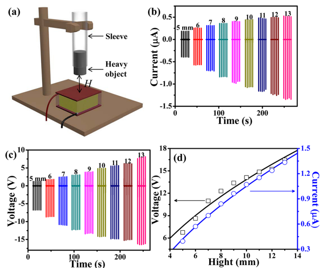
Figure 4. Performance of the NG under different impact forces. (a) Schematic diagram of the drive method. The sleeve is used to make the free-falling object impact the same place in the experiment. (b,c) The current and voltage output of the NG under impact exerted by a free-falling object with different heights, ranging from 5 to 13 mm. (d) Relationship between the peaks of the output voltage (output current) and the height of the free-falling. The square and circle points are experimental data, and the curves are the fitting curves by a square root function.
