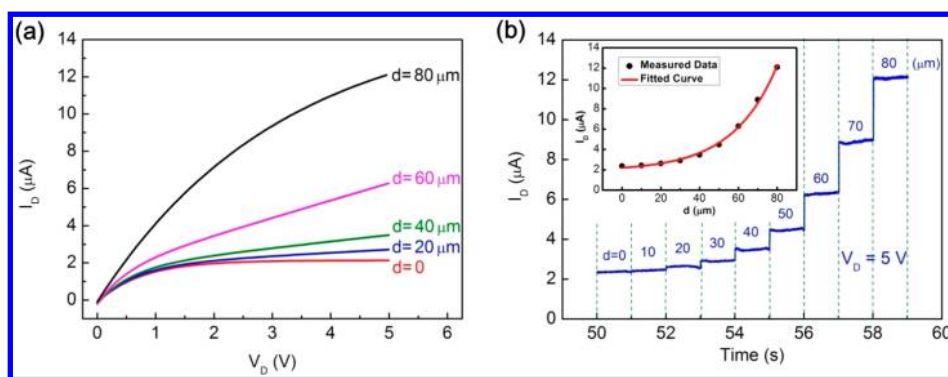
Figure 6. Characteristics of the CE-FET in enhancement mode. (a) I_D – V_D output characteristics with different vertical distances. (b) I_D output characteristics at a drain voltage of 5 V with different vertical distances. The inset is I_D – d transfer characteristics.
