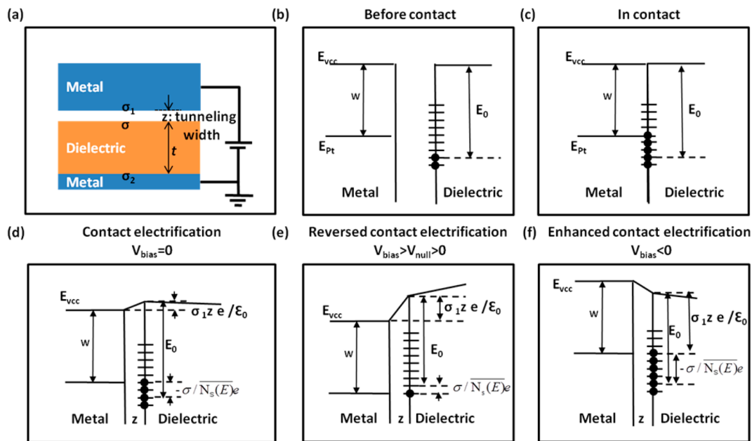
Figure 1. (a) Illustration of the contact electrification process with a tunneling width z , the charge transferred to the dielectric surface with a density of \sigma , induced charge density \sigma_1 and \sigma_2 . (b–f) Energy band diagrams for the metal and dielectric materials in the situations of precontact (b), in contact with no bias (c), in separation equilibrium with no (d), positive (e), and negative (f) bias.
