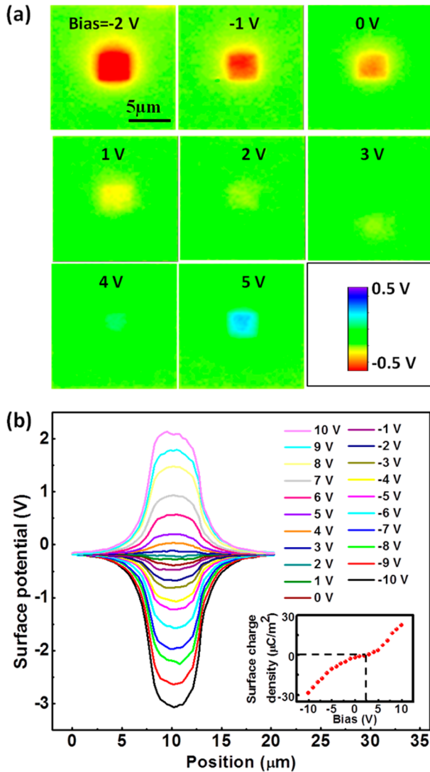
Figure 3. (a) Surface potential distributions of the Parylene film including the areas that were rubbed by Pt coated AFM tip at different bias from -2 to 5 V. (b) Cross section profiles of the surface potential of the Parylene film rubbed with bias from -10 to 10 V. The inset is the calculated surface charge density as a function of bias. With a bias of about 2.5 V, the surface charge density is zero, indicating the contact electrification is completely canceled out by the applied bias.
