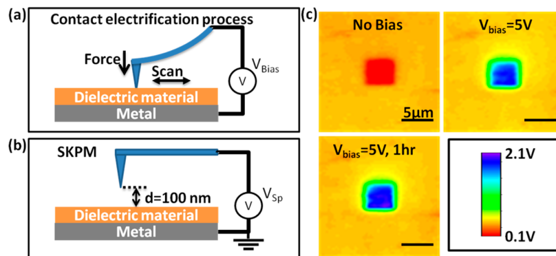
Figure 2. Schematic of experiment setup including two steps: (a) the first step is to use AFM tip with a bias between the tip and the substrate scan over the surface in contact mode, (b) the second step is to use SKPM to map the surface potential distribution. (c) Surface potential distribution of the rubbed and the surrounding area after regionally rubbed by AFM tip at no bias and 5 V bias immediately after rubbing and 1 h later, demonstrating that bias can reverse the triboelectric charge transfer, and the transferred charges have little leakage or diffusion.
