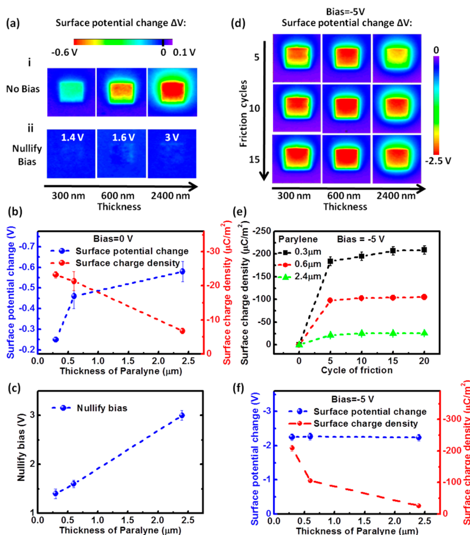
Figure 4. Thickness dependence of contact electrification and bias modulation. (a) Images of surface potential change \Delta V of different thickness samples after they were rubbed at no bias (i) and nullify bias (ii), respectively. (b) The surface potential change and surface charge density as a function of the thickness of the Parylene layer after the sample was rubbed at no bias. (c) The nullify bias as a function of the thickness of the Parylene layer. (d) Images of surface potential change \Delta V of different thickness samples after they were rubbed by different cycles. (e) Calculated surface charge density as a function of friction cycles. (f) The surface potential change and charge density after 20 cycles of friction as a function of thickness of Parylene.
