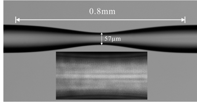
Fig. 1. Microscope image of the abrupt taper with a waist diameter of 57 \mu\text{m} over a length of 0.8 \text{ mm} . The inset shows the grating fringes in the taper. The plane of the image is normal to the axis of the femtosecond laser beam.
