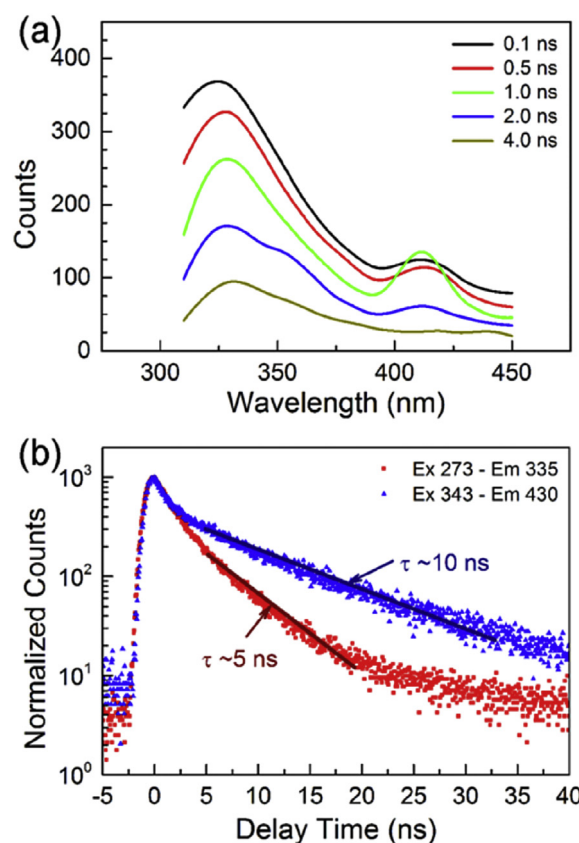
Fig. 5. (a) Time-resolved PL spectra of C-dots after 2 h UV light irradiation at 273 nm excitation. (b) PL dynamics of C-dots after 2 h UV light irradiation at detected wavelengths of 335, 430 nm with 273 and 343 nm excitations, respectively. (A colour version of this figure can be viewed online.)
