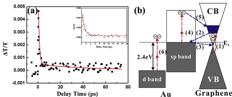
Fig. 5. (a) Femtosecond laser pump-probe result. (b) Energy band schematic diagram of AuNPs/rGO. The insets indicate the enlarged curve. (A colour version of this figure can be viewed online.)
