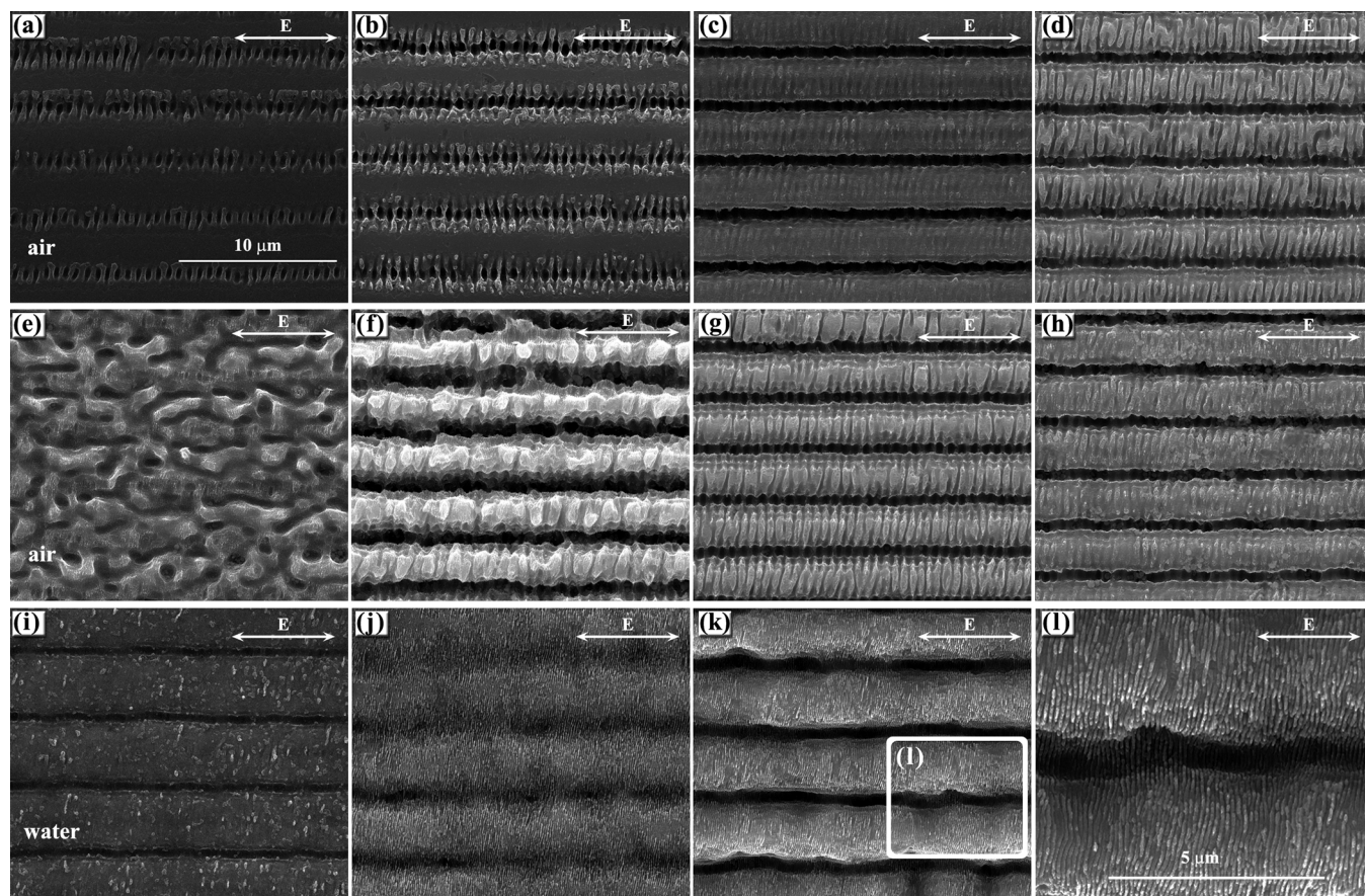
Fig. 3. Evolution of the 2D periodic structures. (a)–(d) are structures fabricated in air at a scanning velocity of 500 \mu\text{m/s} and increasing laser powers of (a) 10.3 mW (b) 15.5 mW (c) 23.1 mW and (d) 30.2 mW. (e)–(h) are the structures fabricated in air at a laser power of 30.1 mW and scanning velocities of (e) 5 \mu\text{m/s} (f) 80 \mu\text{m/s} (g) 250 \mu\text{m/s} and (h) 600 \mu\text{m/s} . (i)–(l) are the structures fabricated in water with laser parameters of (i) 30.2 mW, 300 \mu\text{m/s} (j) 10.2 mW, 5 \mu\text{m/s} and (k) 30.2 mW, 5 \mu\text{m/s} (l) Detailed observation of the region marked in Fig. 3(k).
