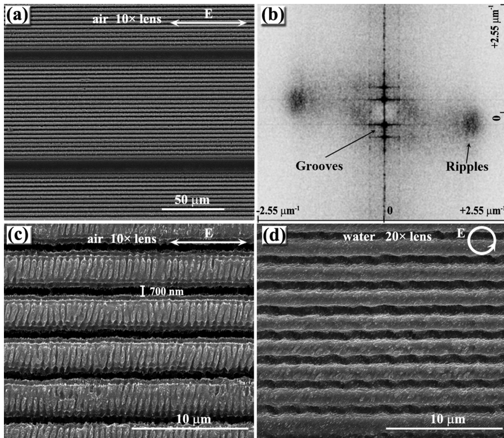
Fig. 2. SEM and 2D-FT images of the 2D periodic structures. (a) Overview of the structures fabricated in air at a laser power of 30.4 mW and a scanning velocity of 150 \mu\text{m/s} . The corresponding 2D-FT image was shown in Fig. 2(b). (c) Enlarged view of the structures shown in Fig. 2(a). (d) Parallel grooves fabricated by a circular polarized laser in water at a power of 31.2 mW and a velocity of 100 \mu\text{m/s} . The corresponding laser polarization direction was marked on each SEM image.
