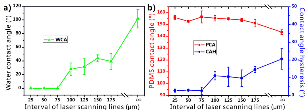
Fig. 6. Influence of \lambda on the wettability of the laser-ablated SSM. (a) Water wettability in air. (b) Underwater wettability of a liquid polymer droplet.
