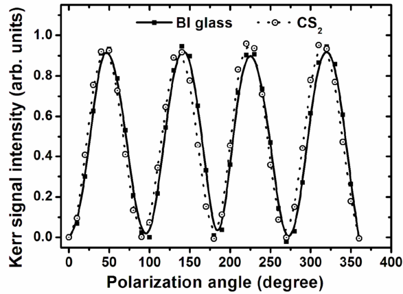
Fig. 5. Polarization dependence of the optical Kerr signals of BI glass and \text{CS}_2 induced by 30-fs pulses.
