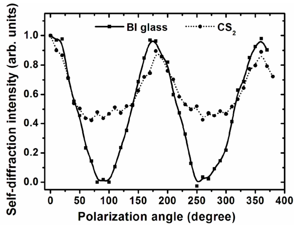
Fig. 4. Polarization dependence of the self-diffraction signals in BI glass and \text{CS}_2 induced by 30-fs pulses.
