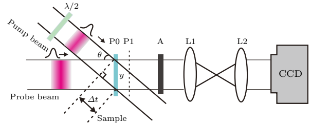
Fig. 1. Schematic diagram of the experimental setup, L1, L2: lens with a focal length of f = 150 \text{ mm} , make up a 4f imaging system. A: analyzer, y : overlap length of probe and pump beams, \Delta t : delay time, P0: the imaging plane of the imaging system; and P1: the plane at 2 cm behind P0.
