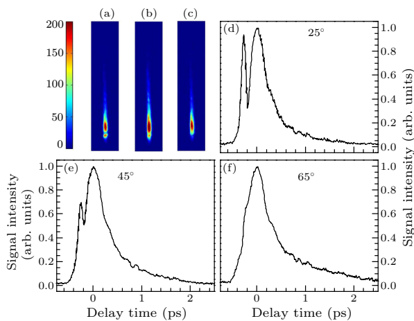
Fig. 5. The recorded signal images with polarization angle kept at (a) 25°, (b) 45° and (c) 65°. (d)–(f) The time-resolved OKG signals of CS 2 by spatial-temporal transformation of the recorded signal images in (a)–(c).
