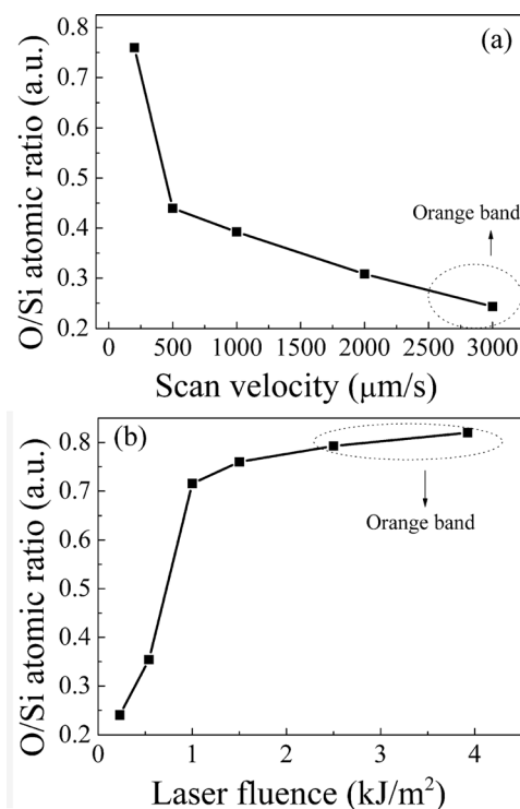
FIG. 3. The atomic ratio of oxygen to silicon in silicon microstructures induced by femtosecond laser for (a) different scan velocities and a laser fluence of 1.5 \text{ kJ/m}^2 and (b) different femtosecond laser fluences and a scan velocity of 200 \text{ }\mu\text{m/s} .
