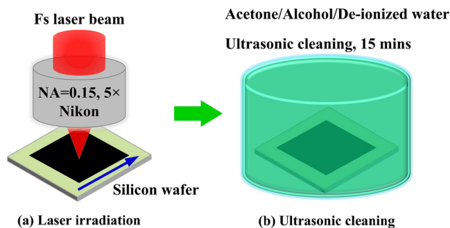
Fig. 1. (Color online) Technological process for fabrication of silicon surface microstructures. (a) Laser irradiation; (b) Ultrasonic cleaning.
