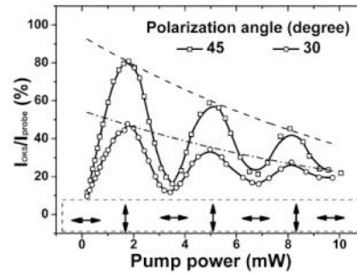
Fig. 1. Pump power dependence of OKS signals in CS 2 when the polarization angle between the pump and probe beams was fixed at 45° and 30°, respectively. The arrows in the rectangle show the polarization directions of the OKS signals at the corresponding pump power. The dashed lines (guided for eyes) show the attenuation trend of peak intensity.
