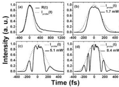
Fig. 2. (a) Temporal profile of 400 nm probe pulse I_{\text{probe}}(t) and nonlinear response of \text{CS}_2 R(t) , and temporal profile of the probe pulse after passing through the OKS setup when the pump power was fixed at (b) 1.7 mW, (c) 5.1 mW, and 8.4 mW, respectively. The dashed lines in (b)-(d) show the temporal profiles of the incident probe pulse I_{\text{probe}}(t) .
