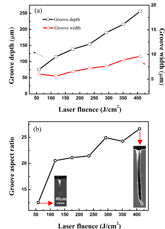
Fig. 5. (a) Depths, widths, and (b) aspect ratios of grooves versus femtosecond laser fluences. The grooves were fabricated by using femtosecond laser irradiation and then etched successively by 20 wt% HF for 60 min and 20 wt% KOH for 20 min.
