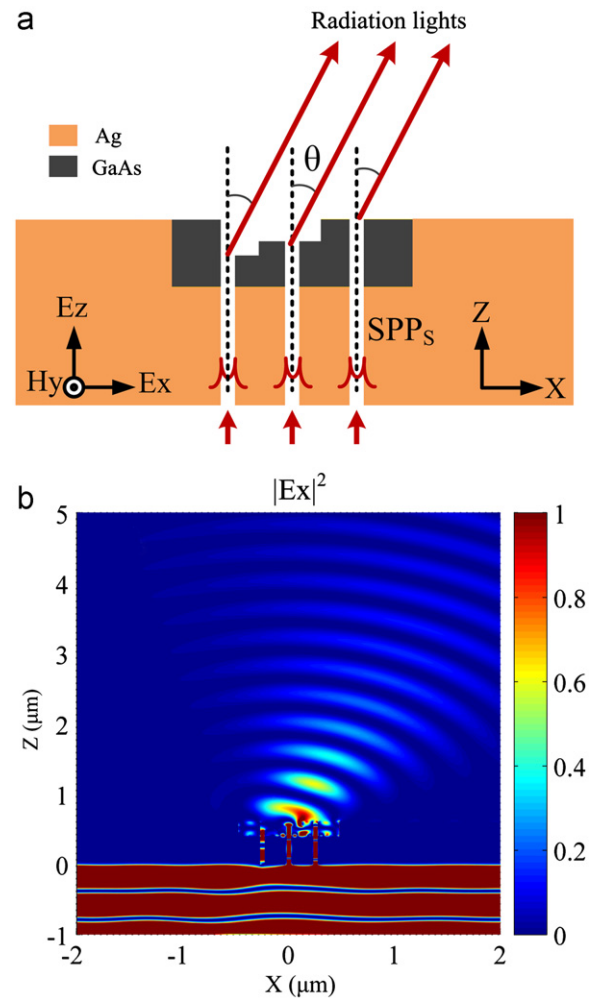
Fig. 7. (a) A schematic drawing of a three-slit composite structure for beam deflection and (b) The simulation result of optical transmission through the structure.
