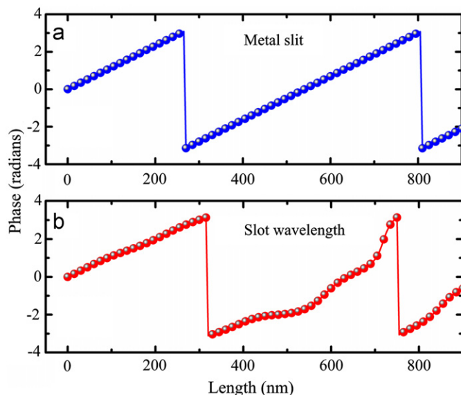
Fig. 6. FDTD simulation results of relative phase at the center of the exit as a function of the waveguide length (a) metal slit and (b) slot waveguide. The width of these both are assumed to be 50 nm.
