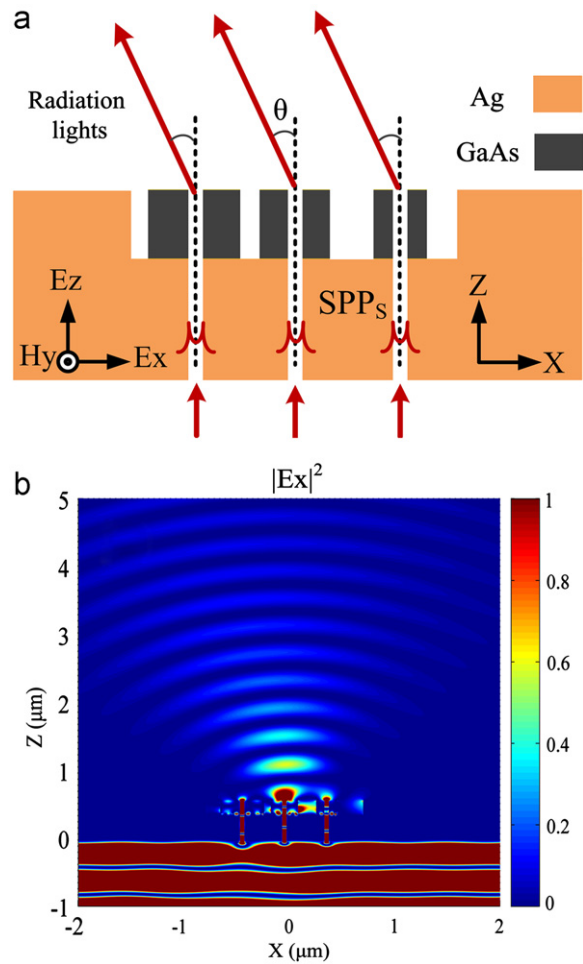
Fig. 4. (a) A schematic drawing of a three-slit composite structure for beam deflection and (b) The simulation results of beam deflection.
