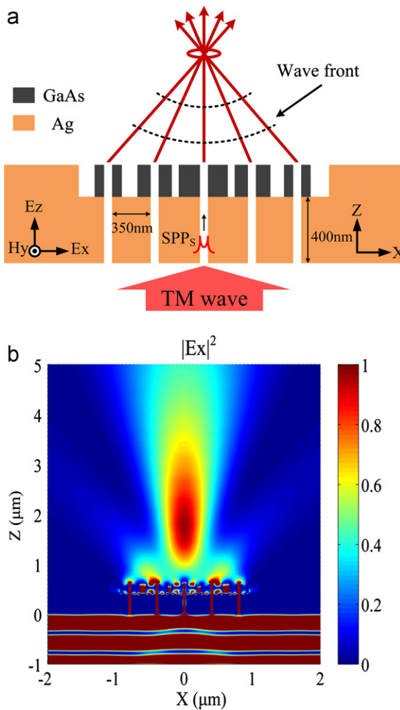
Fig. 5. (a) The schematic of beam focusing structure and (b) The intensity time-average distribution of the focused beam.
