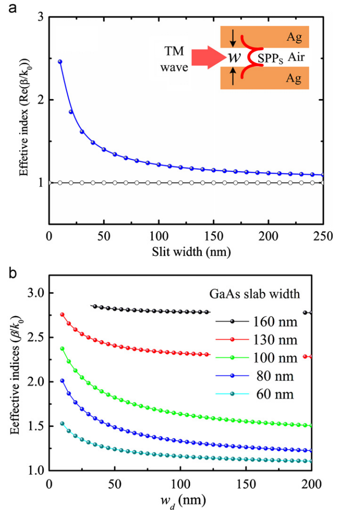
Fig. 2. (a) The effective indices for different slit widths using silver at a wavelength of 800 nm. The dotted line represents the value in air. The inset shows the schematic diagram of the Ag-air-Ag plasmonic waveguide structure and (b) The effective indices versus slot aperture w_d and individual slot wall width d .
