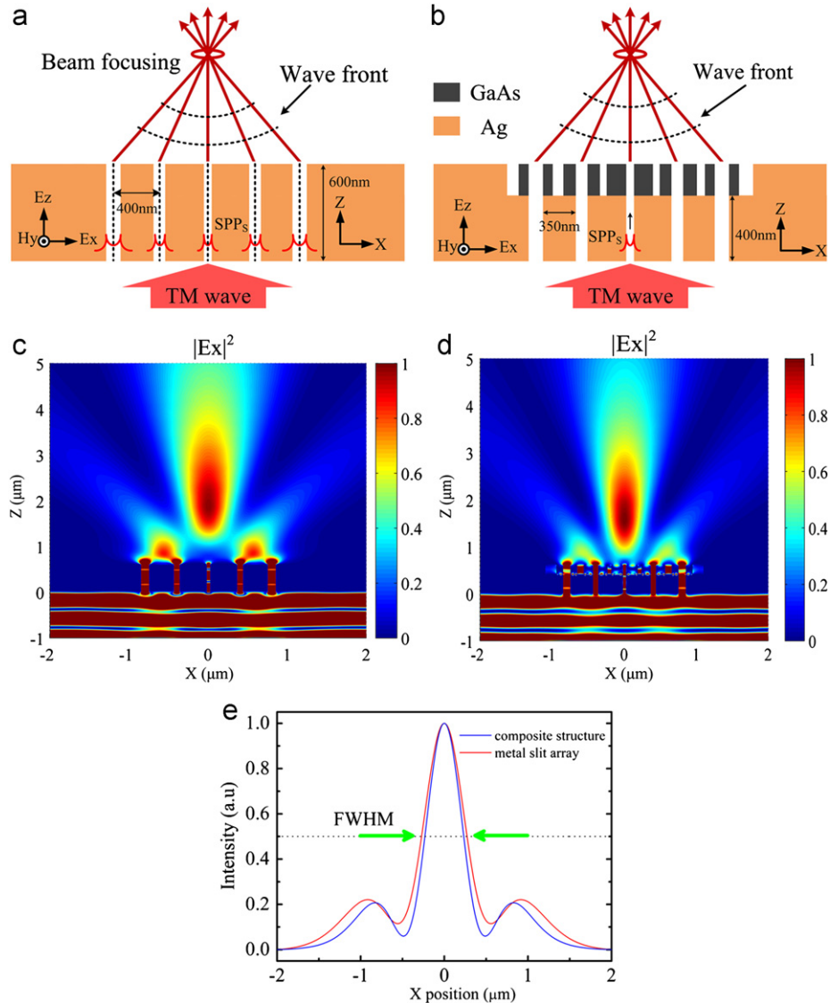
Fig. 3. The schematics of beam focusing structures (a) metal slits with variant widths. (b) composite structure. The normalized intensity distribution of the focused beam from (c) the metal slits with variant widths and (d) the composite structure. (e) Cross-sections plot at the focal planes.
