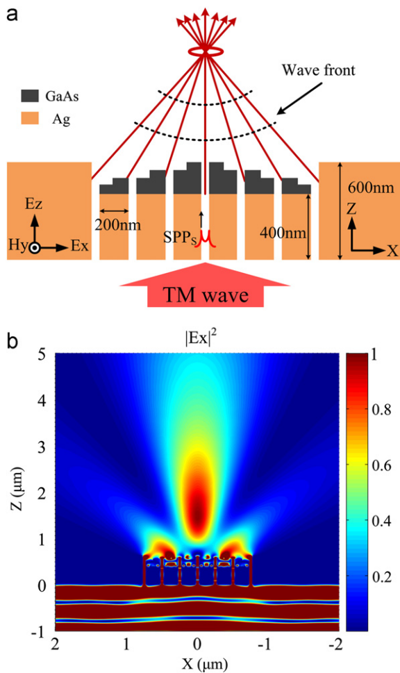
Fig. 8. (a) The schematic of beam focusing structure and (b) The intensity distribution of the focused beam. The slot waveguide length is varied with a 20 nm step profile.
