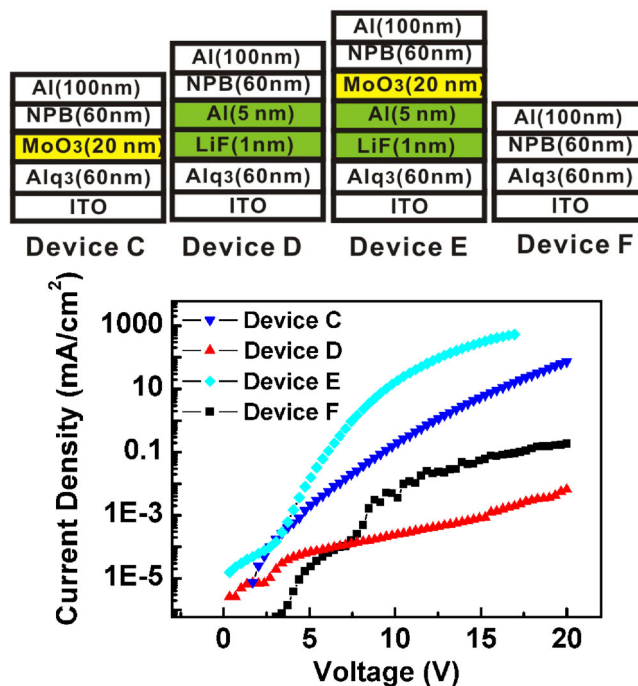
Figure 4 The schematic diagrams of cross-sectional view of device C, device D, device E, and device F, as well as their current–voltage characteristics. Here, ITO was used as the anode, and Al was used as the cathode.
