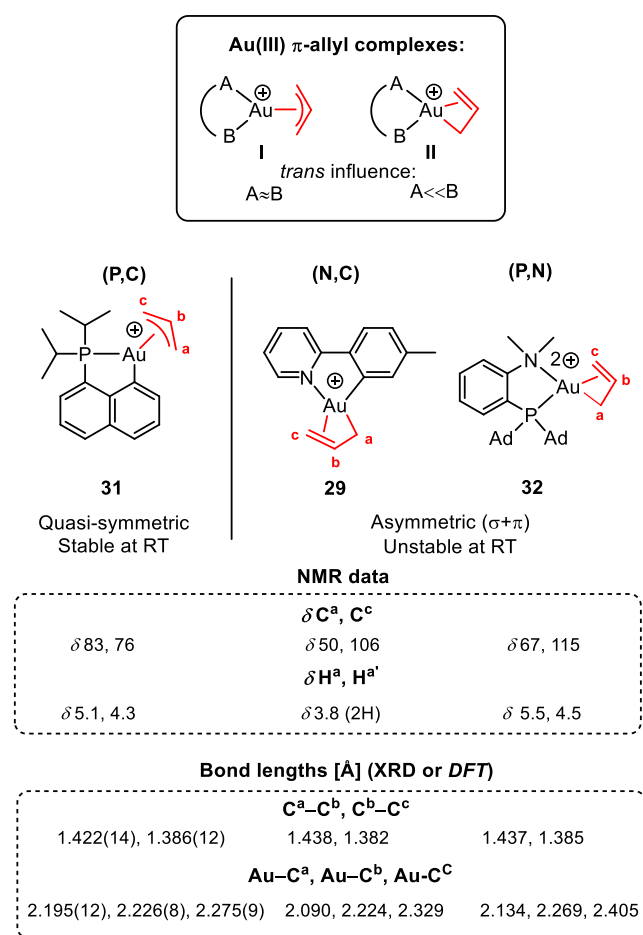
Figure 2. Au(III) \pi -allyl complexes reported by the Tilset group and the Bourissou group. Ad = adamantyl.
