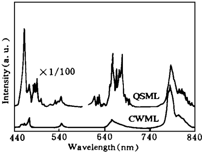
Fig. 2 The spectra of visible lights exiting from a 3 m long Er 3+ -doped fiber pumped by a CW mode-locked laser (bottom) and a Q-switched mode-locked laser (top) with the same average power of 330 mW
