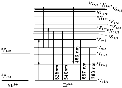
Fig. 1 A simplified energy level diagram of Er 3+ and Yb 3+ ions
