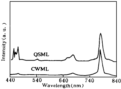
Fig. 3 The spectra of visible lights exiting from a 4.9 m long Er 3+ /Yb 3+ -doped fiber pumped by the CW mode-locked laser (bottom) and the Q-switched mode-locked laser (top) with the same average power of 280 mW
