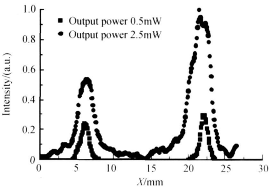
图 3 激光从 27 mm 长的光纤出射后, 光强沿直径的分布情况 Fig.3 Optical intensity distribution along diameter of the output laser from the 27 mm fiber
