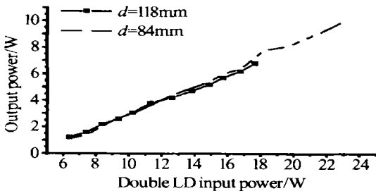
图6 晶体间距离不同时双Nd:YVO 4 激光器的输出功率实验结果 Fig.6 Experiment results of double Nd:YVO 4 laser's output power with different space between two crystals
