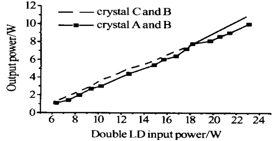
图7 掺杂浓度不同时双Nd:YVO 4 输出功率的实验结果 Fig.7 Double Nd:YVO 4 laser's output power with two crystals have different consistency
