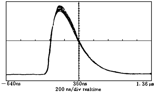
Fig. 4 Frequency-doubled Q-YAG laser pulse (pulse width averaged over 10 pulses is 382.3 ns)
