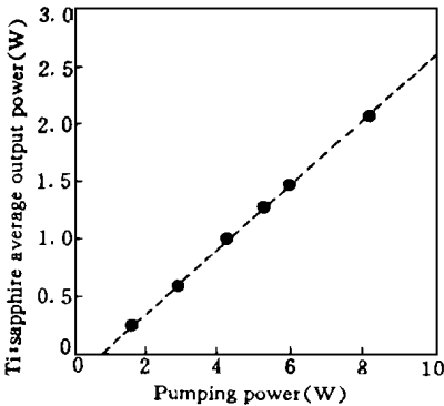
Fig. 3 Measured output power versus pumping power
