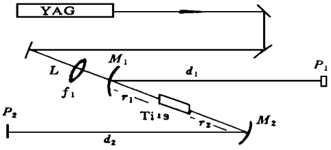
Fig.2 Frequency doubled Q-switched Nd : YAG laser pumped Ti:sapphire laser
