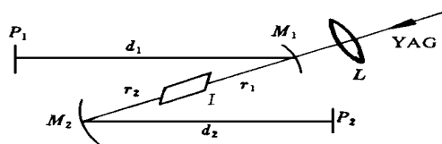
Fig. 1 Schematic diagram of the YAG laser pumped Ti:sapphire laser
