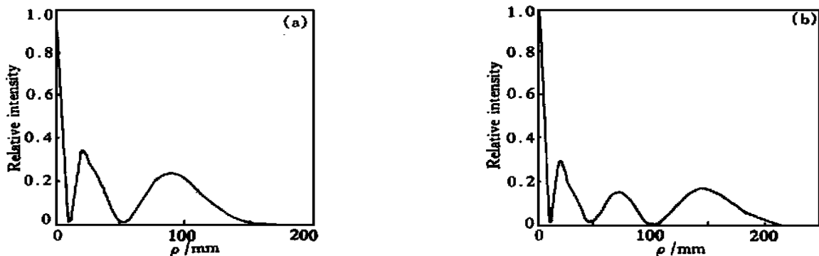
Fig. 4 Calculations of intensity versus radius distribution of the diffraction rings on the observing plan when the sample is located on the focus plan. (a) |\Delta\Psi_0| = 4\pi ; (b) |\Delta\Psi_0| = 6\pi
