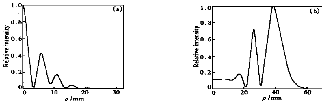
Fig. 3 Intensity versus radius distribution of the diffraction rings on the observing plan, calculated with different sample position z_1 and different \Delta\Psi_0 . (a) z_1 = -25 mm, \Delta\Psi_0 = -4\pi ; (b) z_1 = -15 mm, \Delta\Psi_0 = 6\pi
