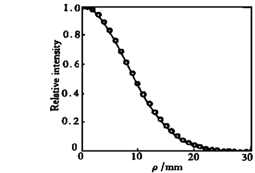
Fig. 2 Comparing calculations of the transverse field distribution of the Gaussian beam in the far field, when \Delta\Psi_0=0 , z_1 assigned any values, respectively using the derived diffraction Eq. (16) (circles) and directly using the Gaussian beam transmission Eq. (1) (line)
