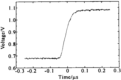
Fig. 6 Response time for probe beam of 520 nm wavelength at rising edge
