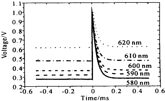
Fig. 10 Experimental result with wavelengths of probe beam at 580 nm~620 nm
