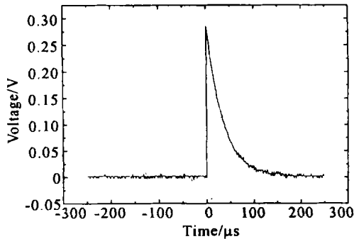
Fig. 4 The curve of YAG laser pulse
