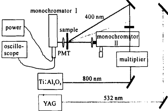
Fig. 3 Schematic diagram of experimental setup for fast optical switch of BR film
