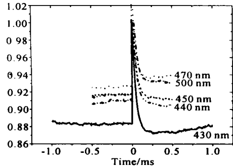
Fig. 8 Experimental result with wavelength of probe beam as 430 nm~500 nm
