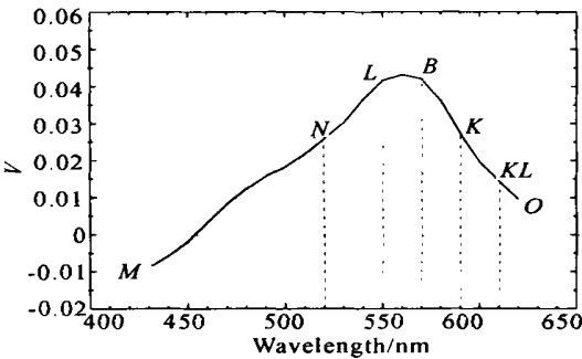
Fig. 11 Relative transmission versus wavelength variation of probe beam
