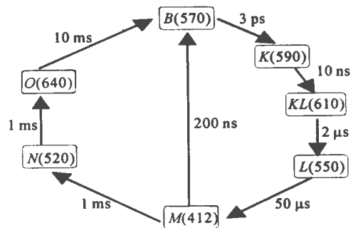
Fig. 1 Schematic diagram of photocycle of BR
