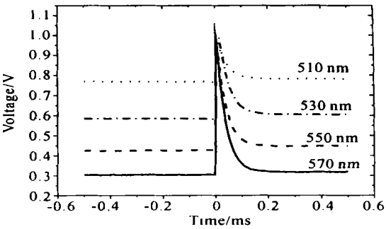
Fig. 9 Experimental result with wavelengths of probe beam at 510 nm~570 nm
