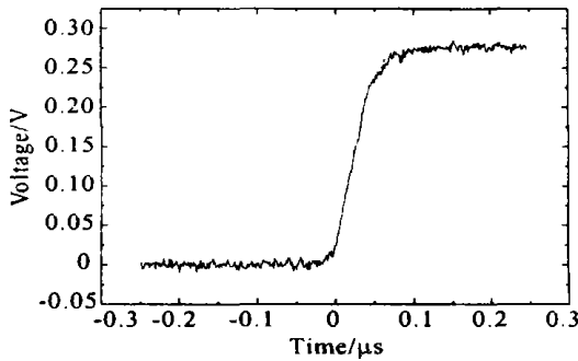
Fig. 4 The curve of YAG laser pulse
