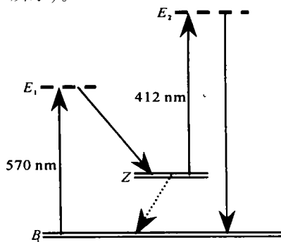
Fig. 2 Simplified energy level diagram of BR
