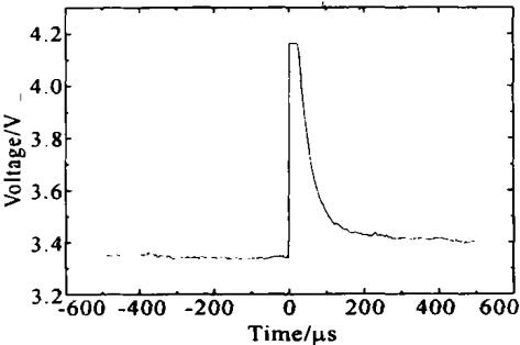
Fig. 7 Experimental result with wavelength of probe beam at 520 nm
