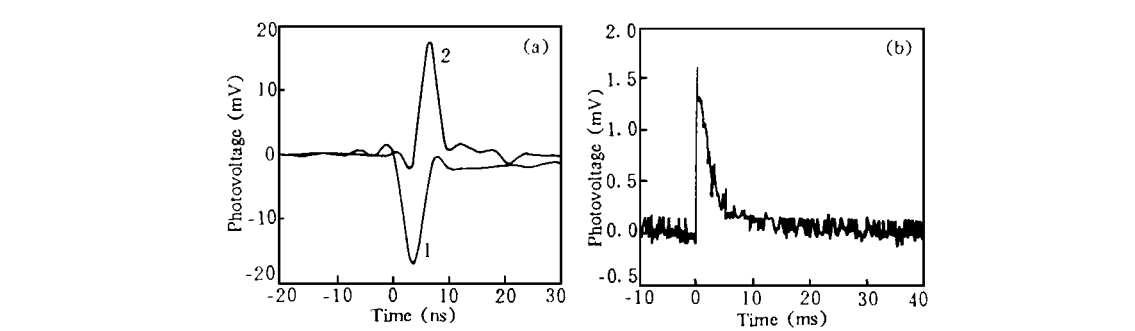
Fig. 3 BR photodetector's response to 30 ps ultrashort laser pulse. 1-BR photodetector, 2-PIN
