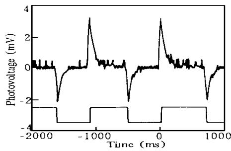
Fig. 5 BR photodetector's differential response to light
