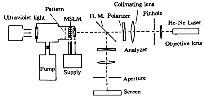
Fig. 3 Experimental arrangement
