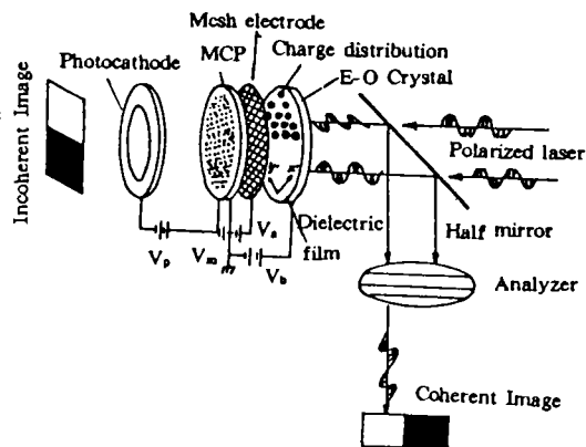
Fig. 1 Operating principle of the MSIM
