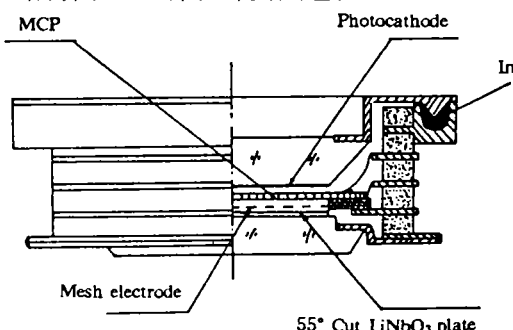
Fig. 2 The proximity-focused microchannel spatial light modulator
