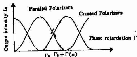
Fig. 5 Polarization readout characteristics as a function of phase retardation
